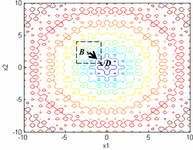
(c) Starting from initial guess \bar{x}_b^2 or point B, the \overline{EA} search converges to \bar{x}_{opt}^2 or point D and f(\bar{x}_{opt}^2) > f(\bar{x}_b^2) . By assuming \rho > 0.75 , \bar{\Delta} is increased in the next iteration.
