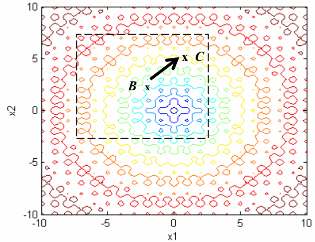
(b) Starting from initial guess \bar{x}_b^2 or B, the \overline{EA} search converges to \bar{x}_{opt}^2 or point C. Since f(\bar{x}_{opt}^2) > f(\bar{x}_b^2) , \rho < 0 and hence \bar{\Delta} is reduced in the next iteration.
