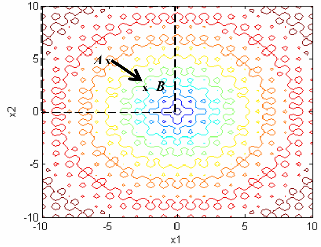
(a) Starting from initial guess \bar{x}_b^1 or point A, the \overline{EA} search converges to \bar{x}_{opt}^1 or point B where f(\bar{x}_{opt}^1) < f(\bar{x}_b^1) . By assuming that \rho > 0.75 , \bar{\Delta} is kept unchanged in the next iteration in the event that \|\bar{x}_{opt}^1 - \bar{x}_b^1\|_\infty < \bar{\Delta}^1 .
