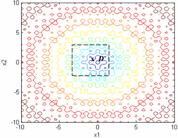
(d) The \overline{EA} search starts from initial guess \bar{x}_b^3 or point D with the increased trust radius.
