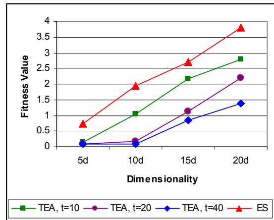
(a) Ackley
