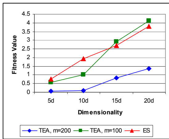
(a) Ackley
