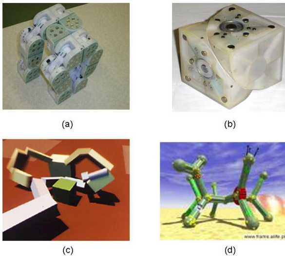
Fig. 10. Examples of physical and simulated modular robots. (a) M-TRAN, (b) Molecube, (c) Karl Sim's Virtual Creature and (d) Framsticks.
