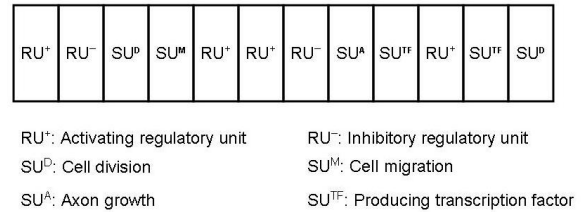
Fig. 17. An example of chromosome for neural development.
