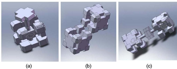
Fig. 11. Mechanical demonstration of CrossCube [63]. (a) The joints; (b) The locks on the boundaries of the modules. (c) Rotation and extension of the joints of the modules.
