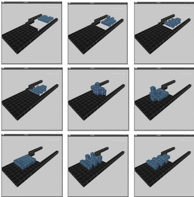
Fig. 14. A set of snapshots demonstrating a series of reconfigurable processes during locomotion and climbing. The robot first adapted its width to the narrow passage, then changed its configuration for climbing up a step, and finally reconfigured itself into a vehicle again to move forward.
