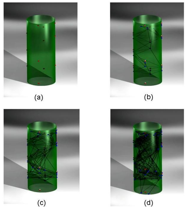
Fig. 19. Development of a nervous system using the GRN model in [41]. (a) A few stem cells are randomly distributed on a hydra-like body wall. (b)-(d) Cells divide, migrate and axons grow. As the development goes on more connections are built up.
