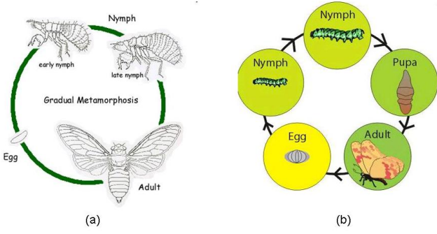
Fig. 3. (a) Incomplete and (b) complete metamorphosis.
